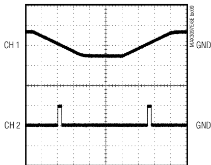
SLEW-RATE FAULT
