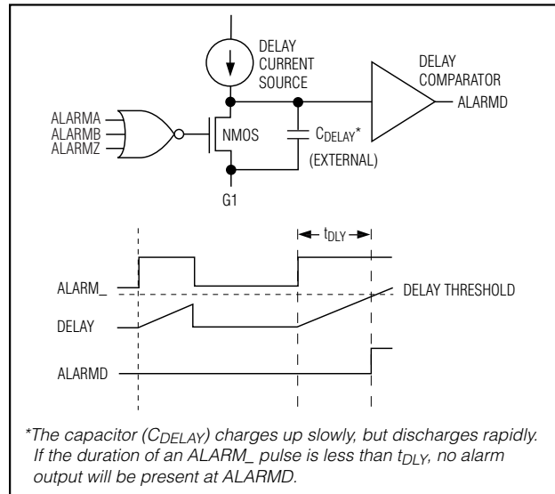
Figure 10. ALARMD Simplified Schematic
