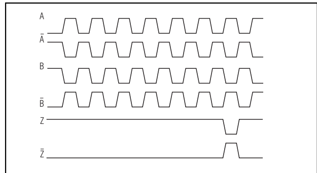
Figure 7. Typical Shaft Encoder Output
