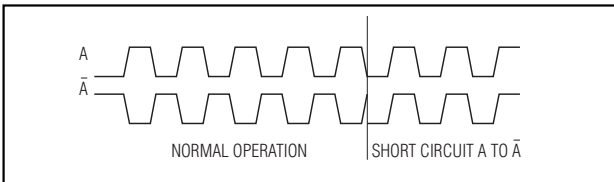
Figure 8. Short-Circuit Detection
