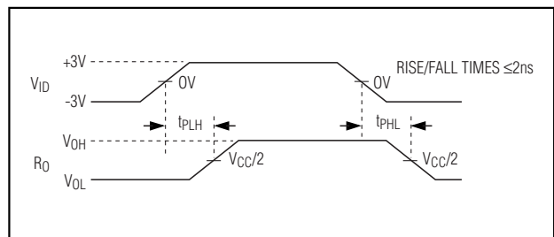
Figure 2. Propagation Delay
