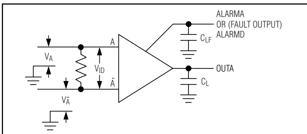
Figure 1. Typical Receiver Test Circuit
