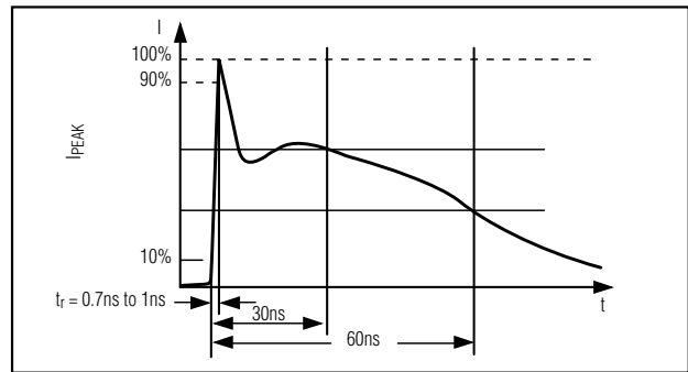
Figure 6b. IEC 1000-4-2 ESD Generator Current Waveform
