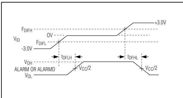
Figure 3. Fault-Detection Timing
