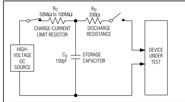
Figure 6a. IEC 1000-4-2 ESD Test Model
