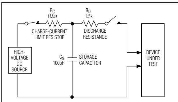
Figure 5a. Human Body ESD Test Model
