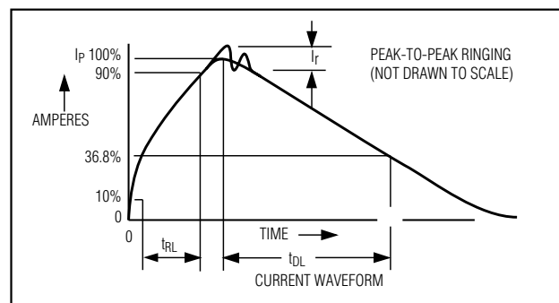
Figure 5b. Human Body Model Current Waveform
