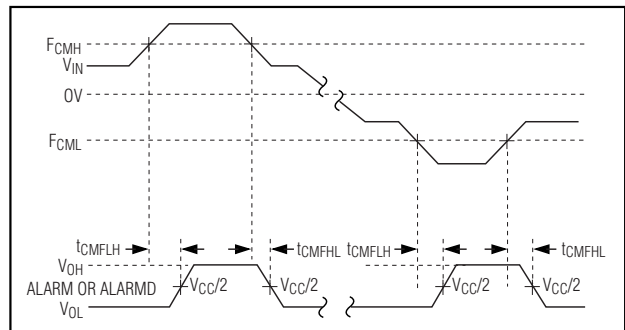
Figure 4. Common-Mode Fault Propagation Delay
