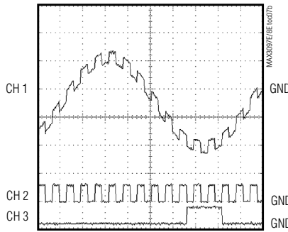
COMMON-MODE VOLTAGE FAULT (LOW SIDE)
