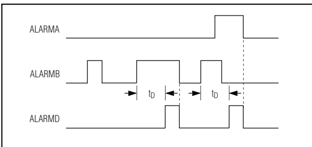
Figure 9. Delayed Alarm Output
