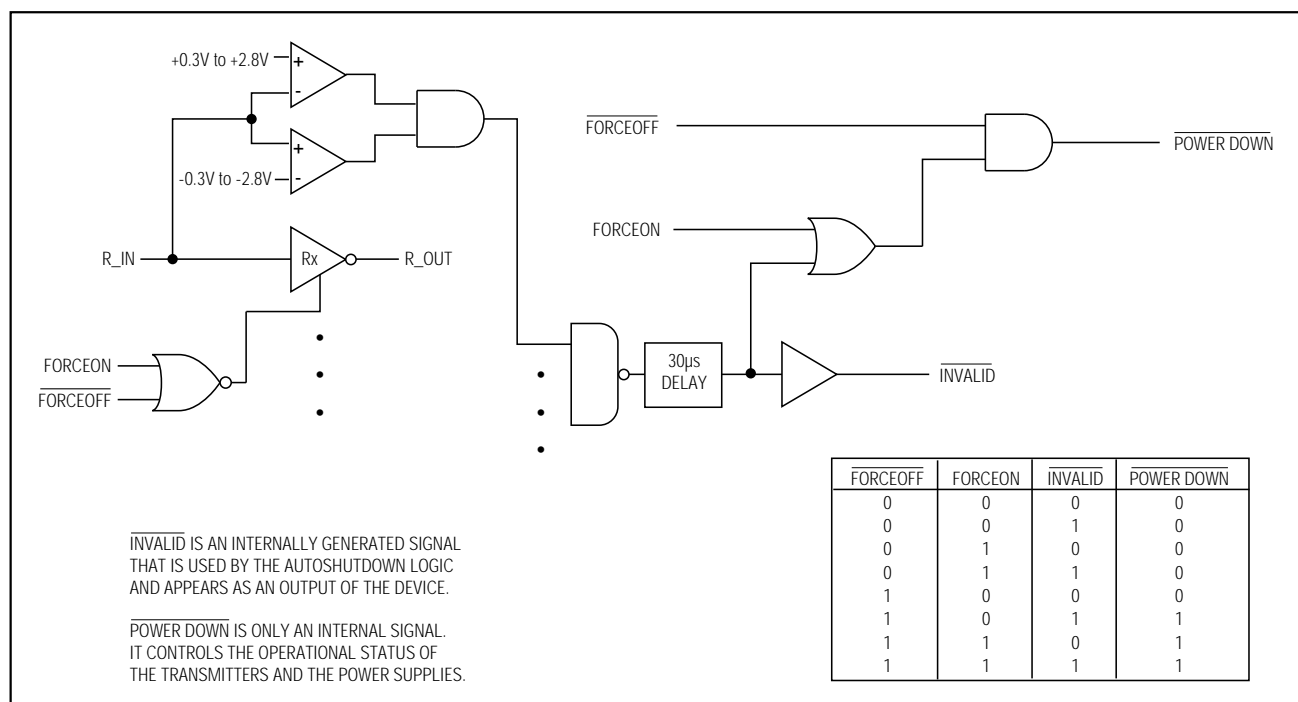
Figure 3. AutoShutdown Logic
