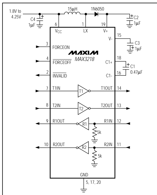
Figure 1. Typical Operating Circuit
