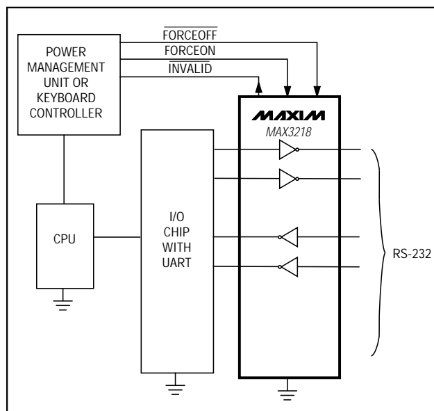
Figure 2. Interface Under Control of PMU
