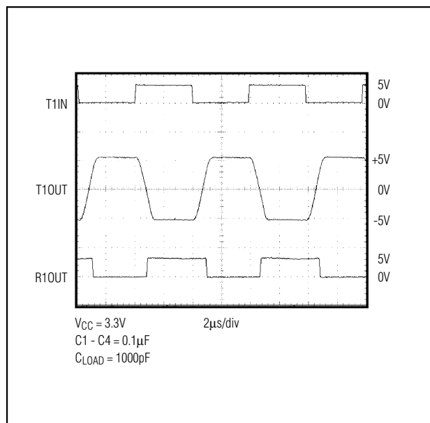
Figure 8. Loopback Test Result at 250kbps
