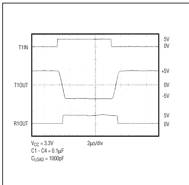
Figure 7. Loopback Test Result at 120kbps
