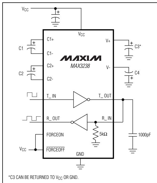
Figure 6. Loopback Test Circuit
