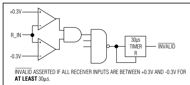
Figure 3a. \overline{\text{INVALID}} Functional Diagram, \overline{\text{INVALID}} Low
