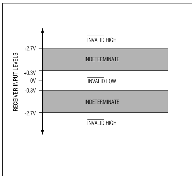
Figure 4a. Receiver Positive/Negative Thresholds for \overline{\text{INVALID}}
