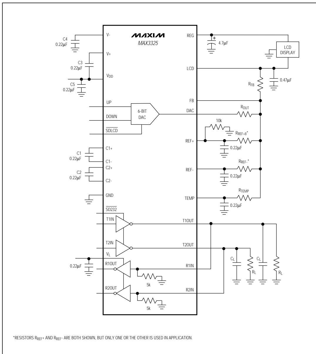
Figure 1. Application Circuit
