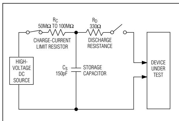
Figure 5. IEC 1000-4-2 ESD Test Model
