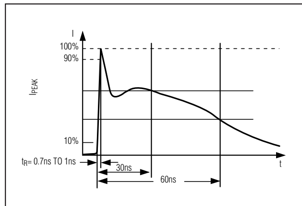
Figure 6. IEC 1000-4-2 ESD Generator Current Waveform
