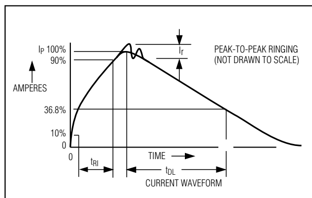
Figure 4. Human Body Model Current Waveform
