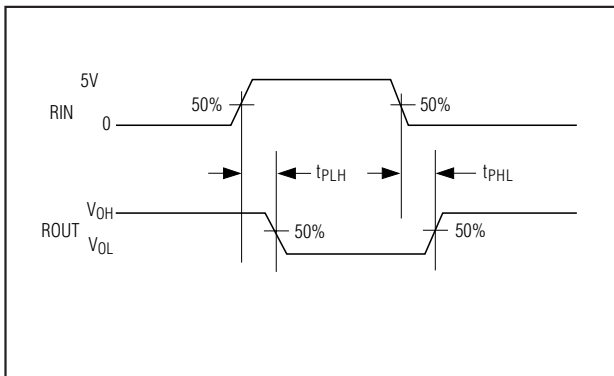
Figure 1. Receiver Propagation-Delay Timing
