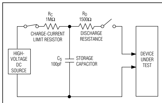
Figure 3. Human Body ESD Test Model
