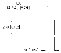
[B] RECOMMENDED SOLDER PAD LAYOUT
