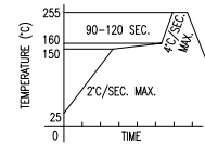
[B] LEAD FREE REFLOW PROFILE
