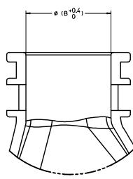
Partial Y-Y SCALE 5:1 WITHOUT RIBS
