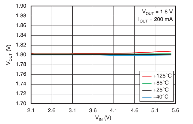
Figure 2. Line Regulation
