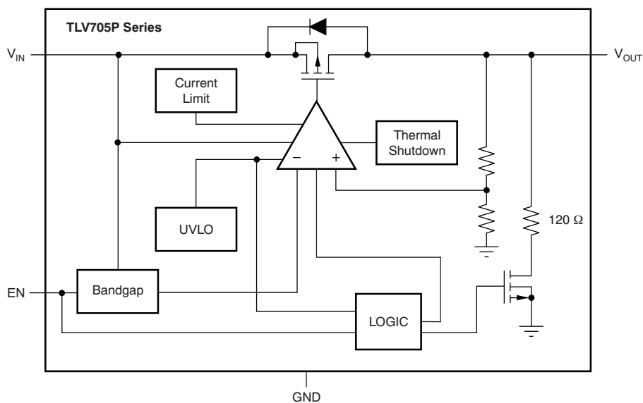
Figure 27. TLV705P Series
