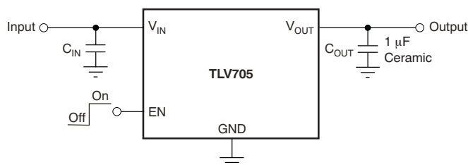
Figure 28. Typical Application Circuit (Fixed-Voltage Versions)
