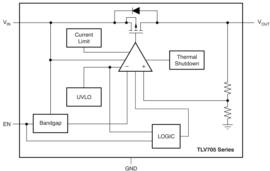
Figure 26. TLV705 Series
