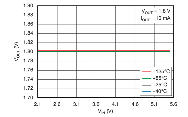
Figure 1. Line Regulation
