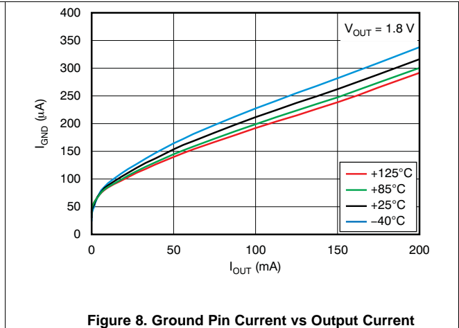
Figure 8. Ground Pin Current vs Output Current
