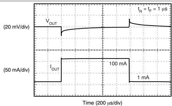
Figure 16. Load Transient 0
