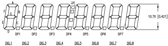
CHARACTER DETAIL
