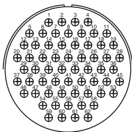
Insert Arrangement 40-82 Service Rating A Number of Contacts 62 Contact Size 16
