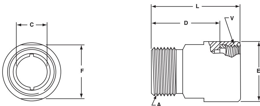
10-113196-XX adapter
