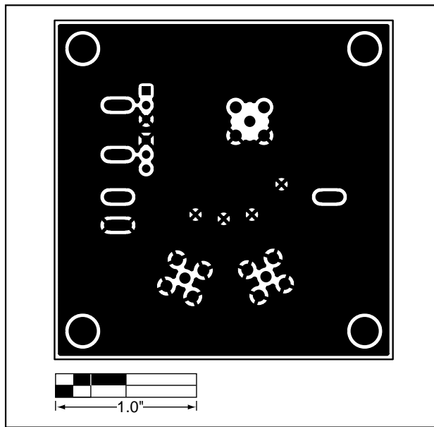
Figure 4. MAX4313 EV Kit PC Board Layout Guide—Solder Side
