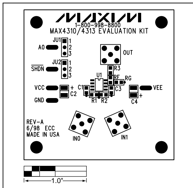
Figure 2. MAX4313 EV Kit Component Placement Guide—Component Side
