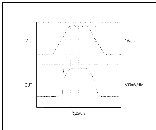
Figure 8. Power-Up/Down Output Voltage
