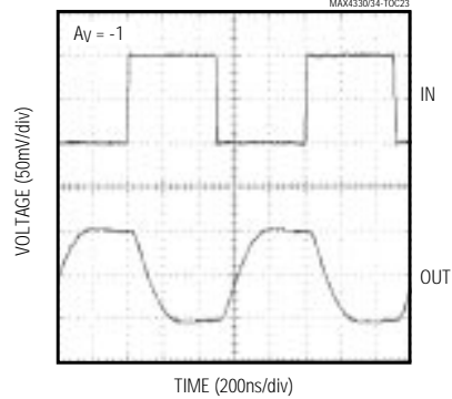
SMALL-SIGNAL TRANSIENT RESPONSE (INVERTING)
