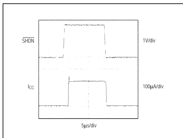
Figure 11. Shutdown Enable/Disable Supply Current
