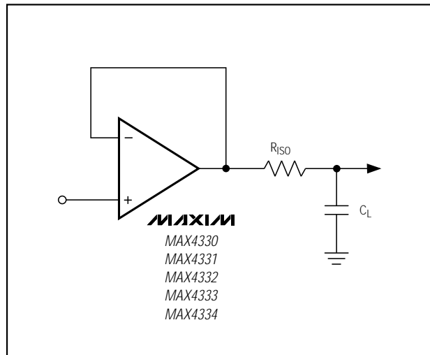
Figure 6. Capacitive-Load-Driving Circuit
