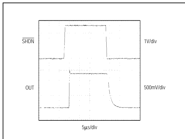
Figure 10. Shutdown Output Voltage Enable/Disable
