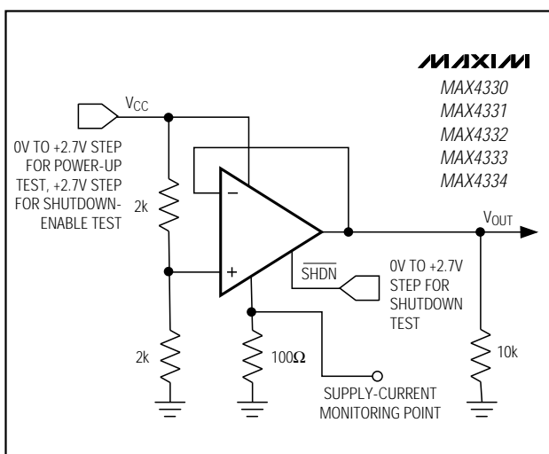
Figure 7. Power-Up/Shutdown Test Circuit
