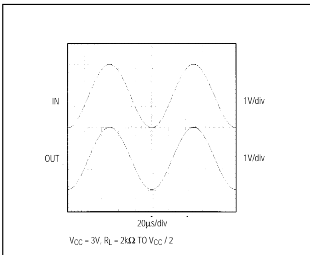
Figure 3. Rail-to-Rail Input/Output Voltage Range
