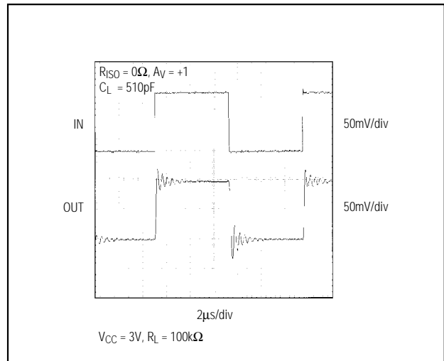
Figure 4. Small-Signal Transient Response with Excessive Capacitive Load
