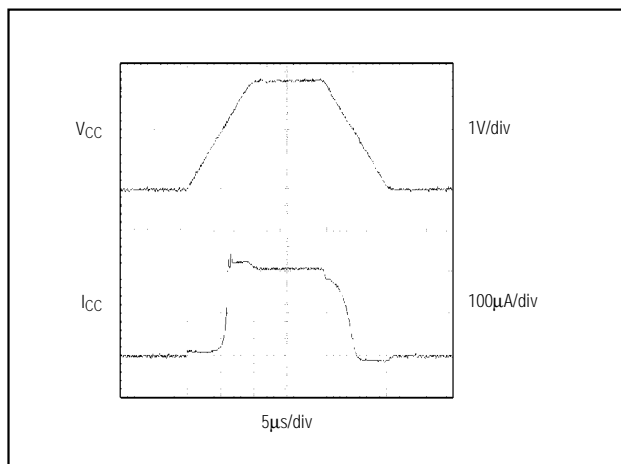
Figure 9. Power-Up/Down Supply Current
