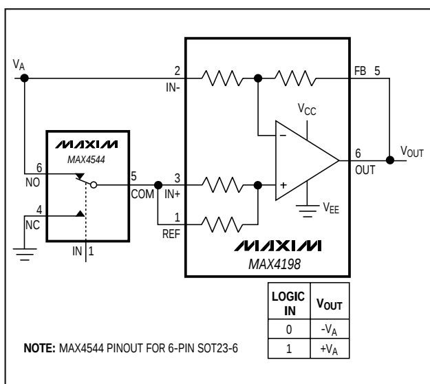
Figure 6. Digitally Controlled Precision Gain of \pm 1 Amplifier
