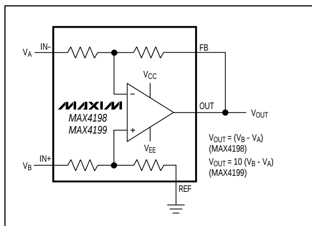
Figure 2. Standard Difference Amplifier
