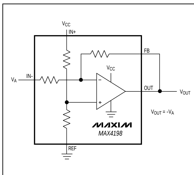
Figure 5. Single-Supply Inverting Amplifier Biased at V_{CC} / 2
