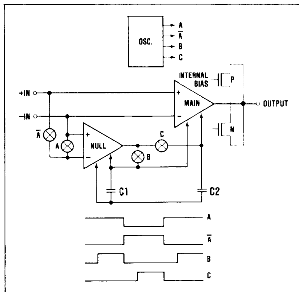
Figure 2. Maxm MAX430 Series Amplifier Block Diagram
