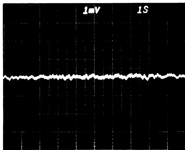
Figure 3. D.C. to 1Hz Noise, 1μV/vert. div. referred to input, 1 second/horiz. div.
