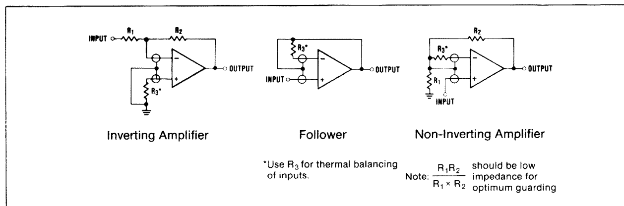
Figure 4. Input Guard Connections
