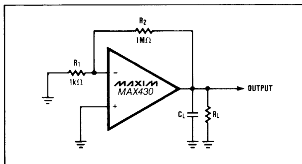
Figure 1. Test Circuit
