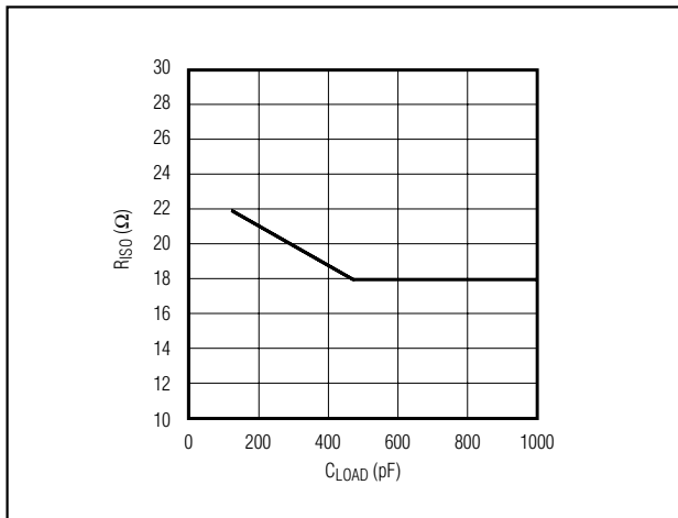
Figure 2. Capacitive Load vs. Isolation Resistance
