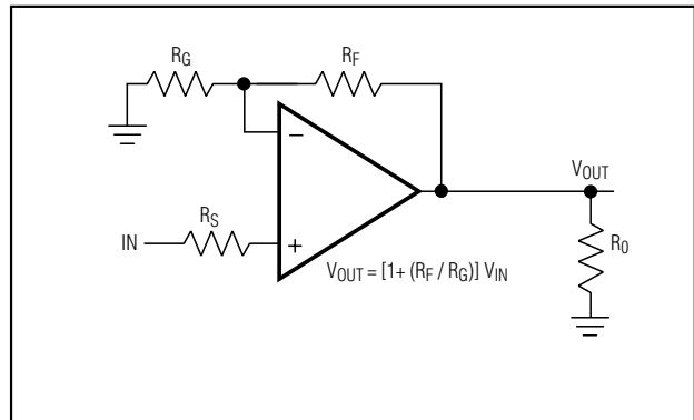
Figure 3a. Noninverting Gain Configuration
