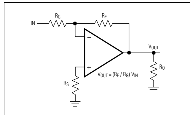
Figure 3b. Inverting Gain Configuration
