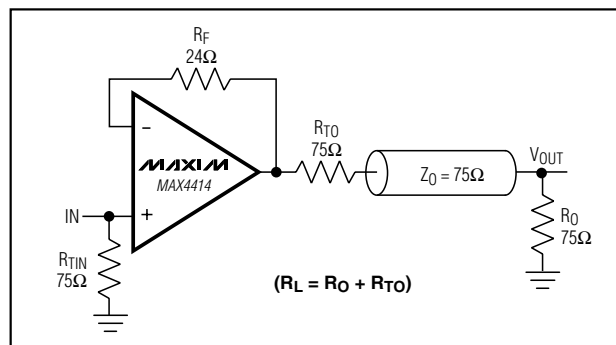
Figure 4. Video Line Driver
