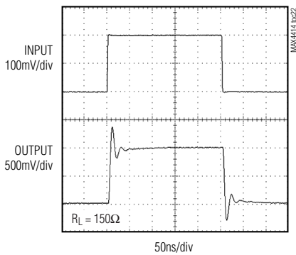
MAX4415/MAX4417/MAX4419 SMALL-SIGNAL PULSE RESPONSE ( C_{LOAD} = 15pF )
