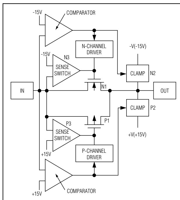
Figure 1. Simplified Internal Structure
