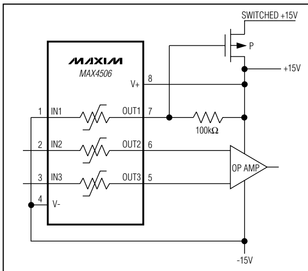
Figure 4. Power-Supply Sequencing
