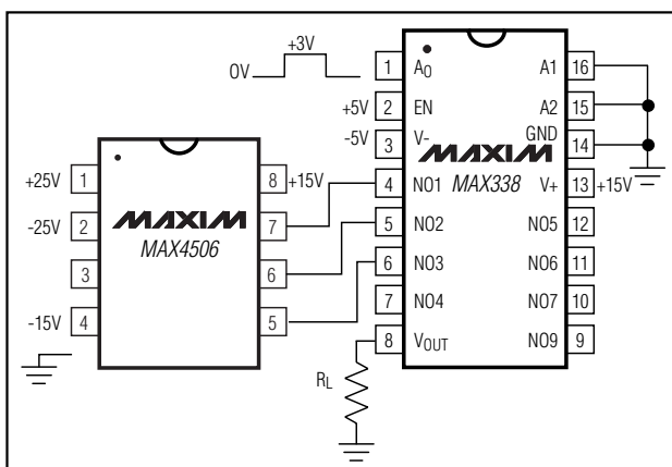
Figure 5. Protecting a MAX338 with a MAX4506
