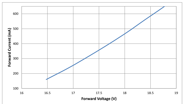
Forward Current vs. Forward Voltage @ 85°C
