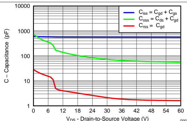
Figure 5. Capacitance
