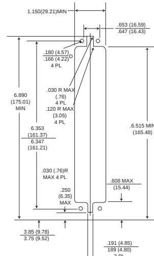
Panel Cutout
