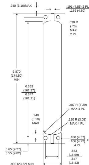
Panel Cutout
