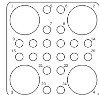
24T4** 20 #20, 4 #8 TRIAX
