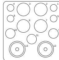
13W2 4 #20, 4 #12, 3 #16 2 #5 COAX
