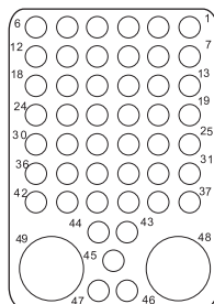
49T2** 47 #20 2 #8 TRIAX
