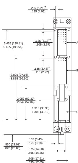
Retainer Plate Detail
