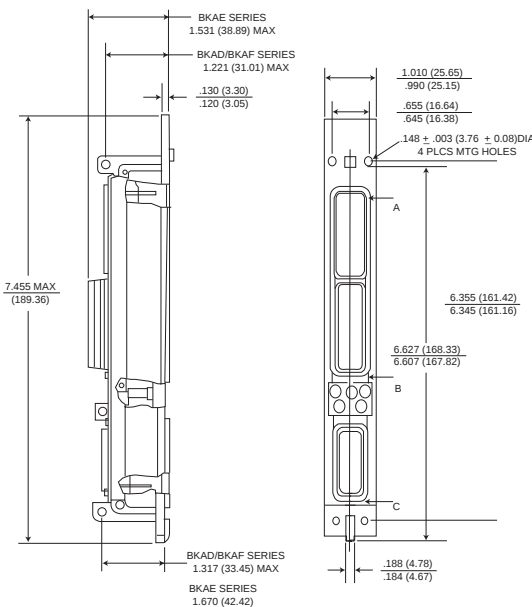
Size 1 Receptacle
