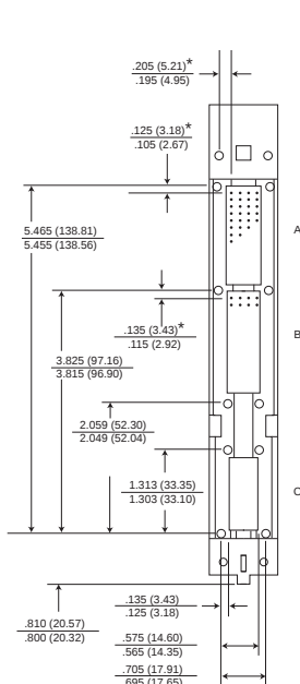
Retainer Plate Detail
