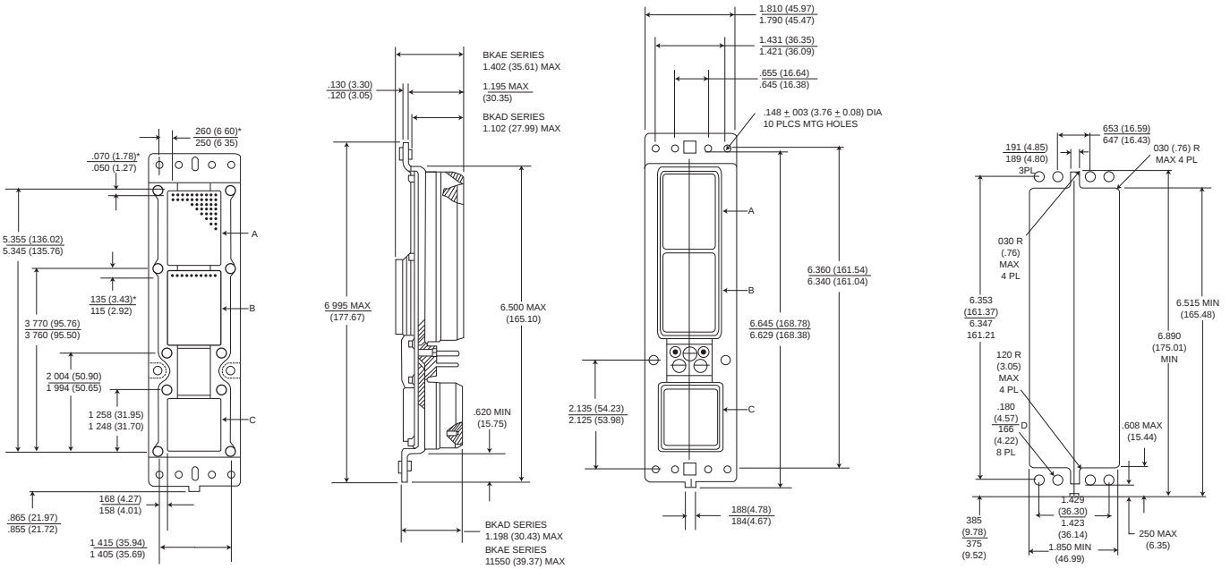
Panel Cutout
