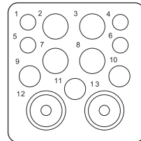
13W2 4 #20 3 #16 4 #12 2 #5 COAX
