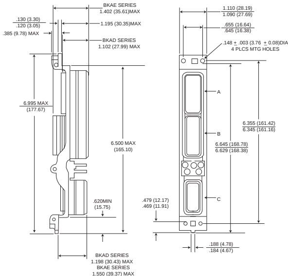
Size 1 Plug
