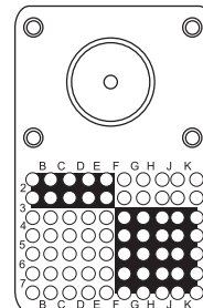
71W1B 70 #22 1 #1 COAX
