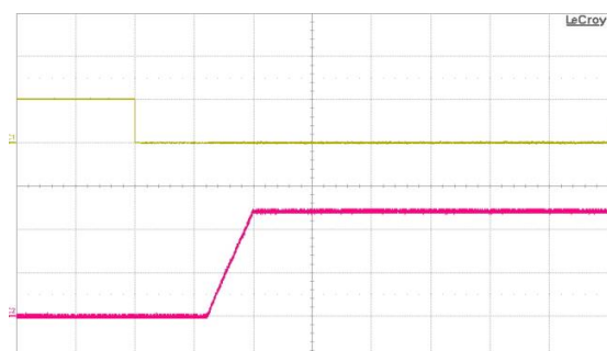
Fig. 9: Turn-on transient at full rated load current (resistive) with C_{out} 10 \mu\text{F} tantalum + 1 \mu\text{F} ceramic at V_{in} = 48\text{V} , triggered via ON/OFF pin. Top trace: ON/OFF signal (5 V/div.). Bottom trace: output voltage (5 V/div.). Time scale: 50 ms/div.
