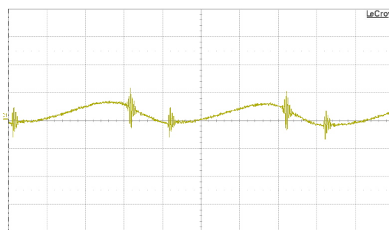
Fig. 16: Input reflected ripple current, i_s (20 mA/div.), measured through 10 \mu H at the source at full rated load current and V_{in} = 48 V
