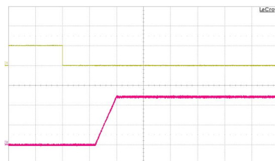
Fig. 10: Turn-on transient at full rated load current (resistive) plus 4700 \mu\text{F} at V_{in} = 48\text{V} , triggered via ON/OFF pin. Top trace: ON/OFF signal (5 V/div.). Bottom trace: output voltage (5 V/div.). Time scale: 50 ms/div.
