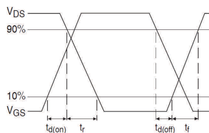
Fig 17b. Switching Time Waveforms
