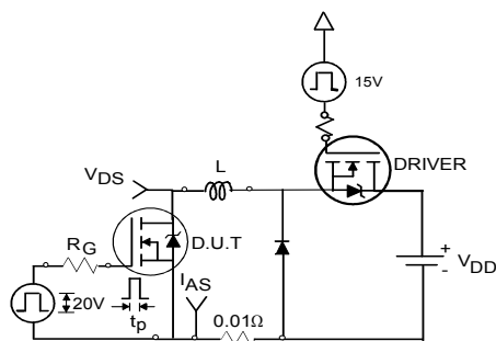
Fig 16a. Unclamped Inductive Test Circuit
