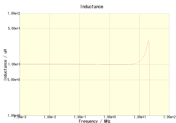
VLF403212MT-100M-CA
