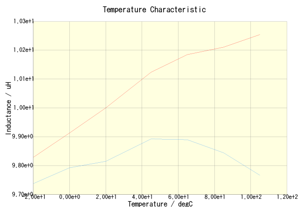
VLF403212MT-100M-CA(DC = 0A)
