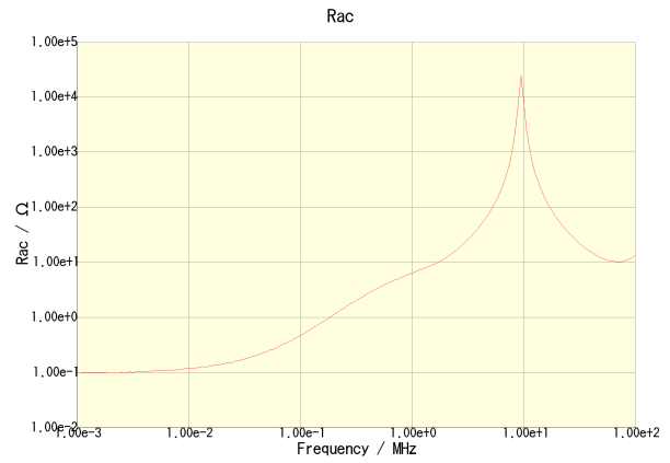
CLF6045T-330M-CA
