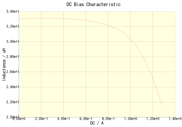
CLF6045T-330M-CA(Amb. Temp. = 20degc)
