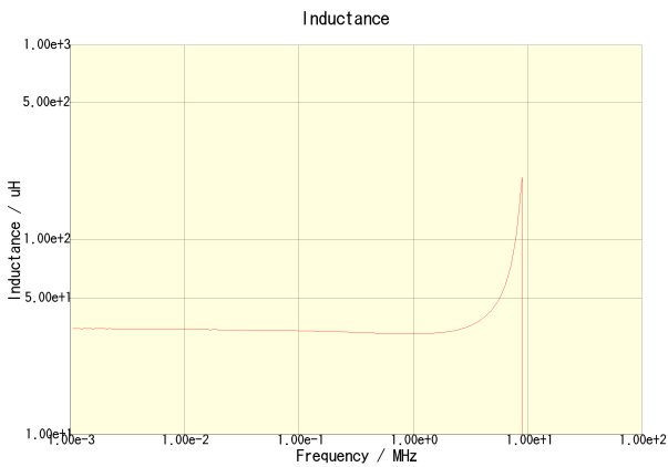
CLF6045T-330M-CA
