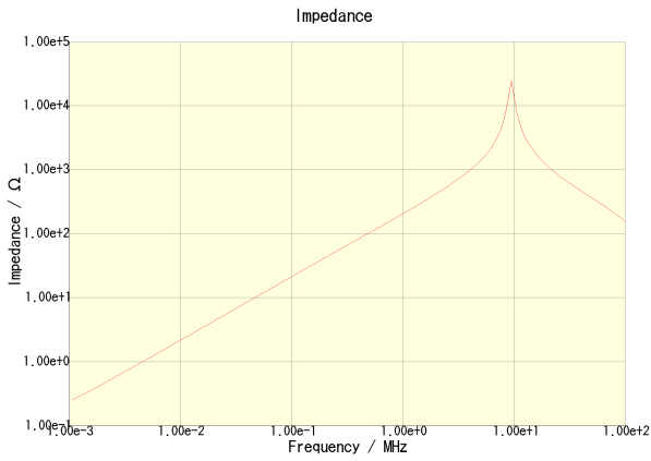
CLF6045T-330M-CA
