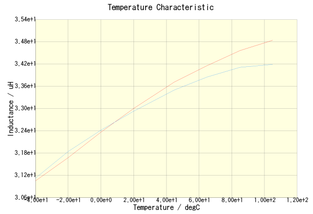
CLF6045T-330M-CA(DC = 0A)
