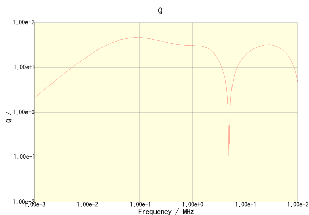
CLF6045T-680M-CA
