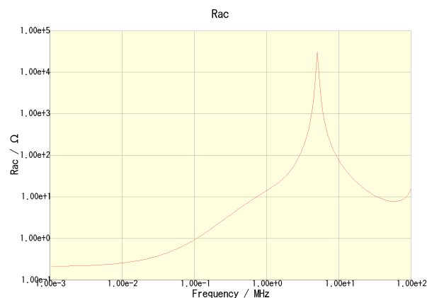
CLF6045T-680M-CA
