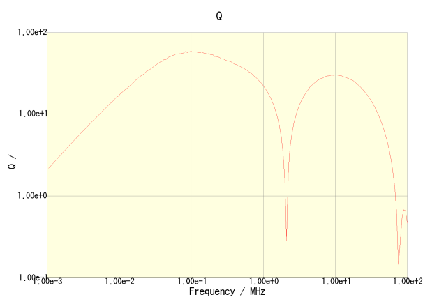
CLF6045T-331M-CA
