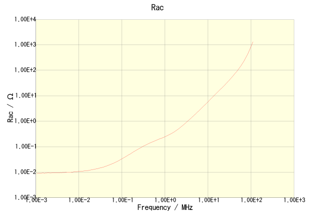
CLF7045T-1R5N-CA
