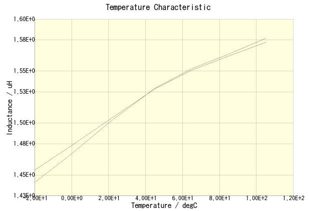
CLF7045T-1R5N-CA(DC = 0A)
