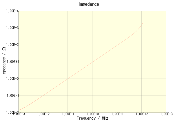
CLF7045T-1R5N-CA
