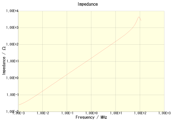
CLF7045T-2R2N-CA
