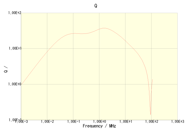
CLF7045T-2R2N-CA
