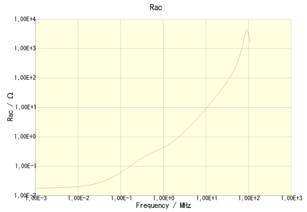
CLF7045T-2R2N-CA
