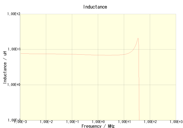
CLF7045T-6R8N-CA
