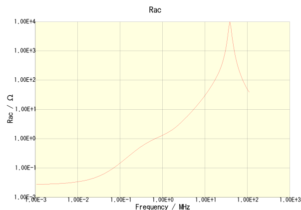
CLF7045T-6R8N-CA
