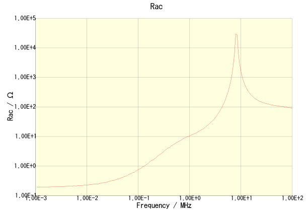
CLF7045T-680M-CA
