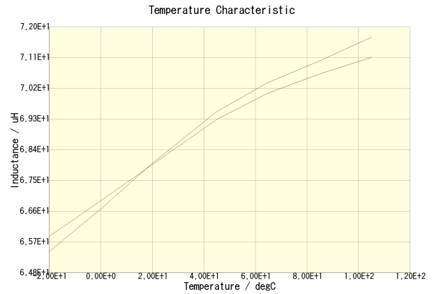
CLF7045T-680M-CA(DC = 0A)
