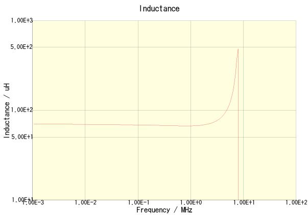
CLF7045T-680M-CA
