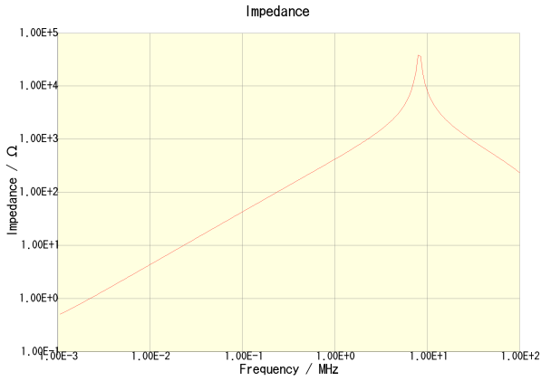
CLF7045T-680M-CA
