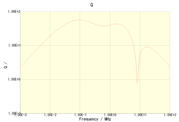
CLF7045T-680M-CA
