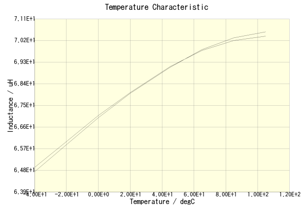
CLF1255T-680M-CA(DC = 0A)
