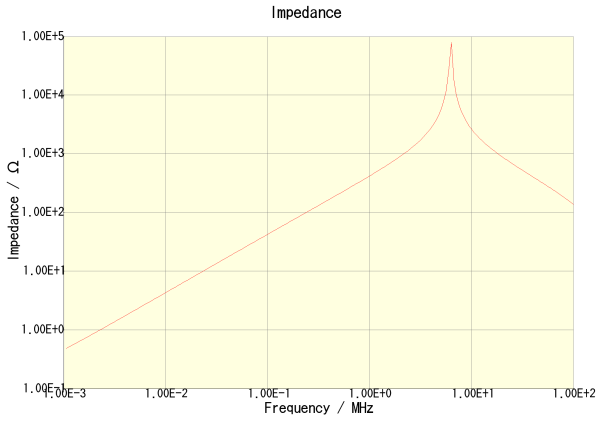
CLF12555T-680M-CA
