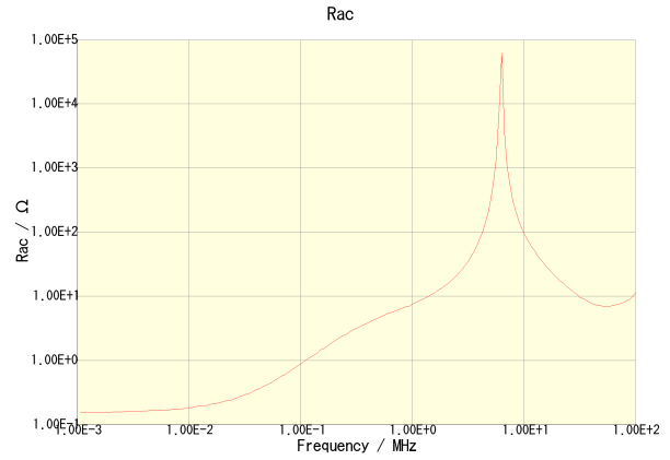
CLF12555T-680M-CA
