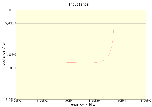
CLF12555T-680M-CA
