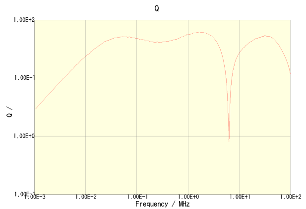
CLF12555T-680M-CA
