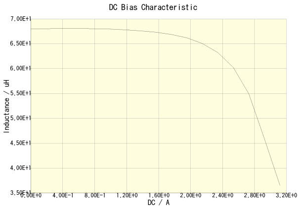
CLF1255T-680M-CA(Amb. Temp. = 20degc)
