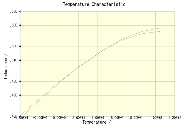
CLF12555T-151M-CA(DC = 0A)
