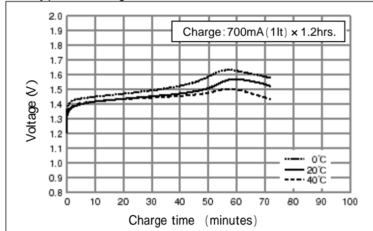
Typical charge characteristics
