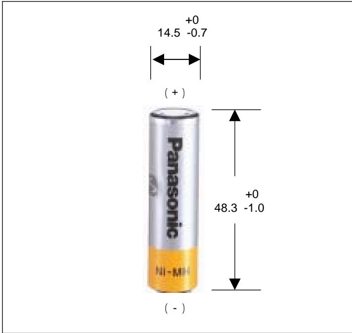
Dimensions (with tube) (mm)
