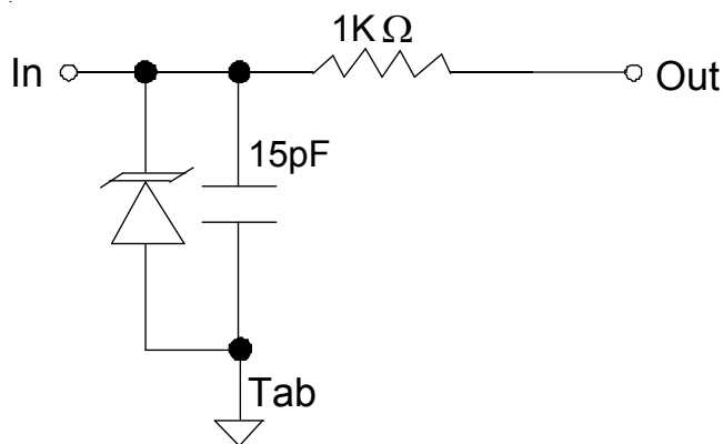
Circuit Diagram
