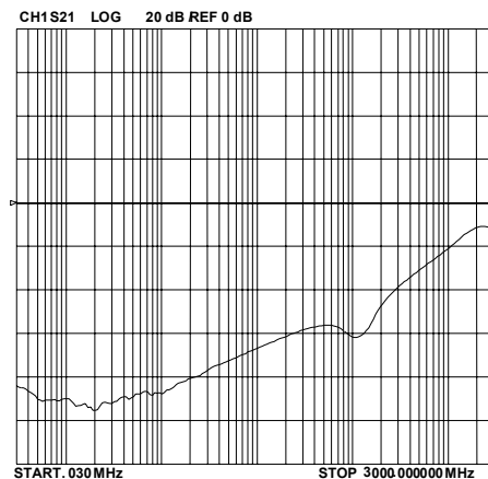
Analog Crosstalk (Each Line)
