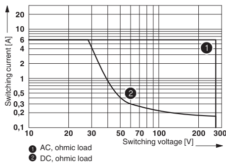
Interrupting rating
