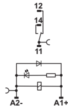
DC coils
