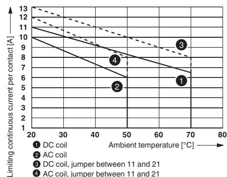
Contact derating
