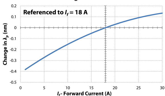
Peak Wavelength vs Forward Current
