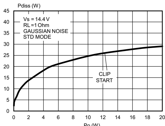
Figure 21. Power dissipation vs. Po (1 Ω, STD mode, audio program simulation)
