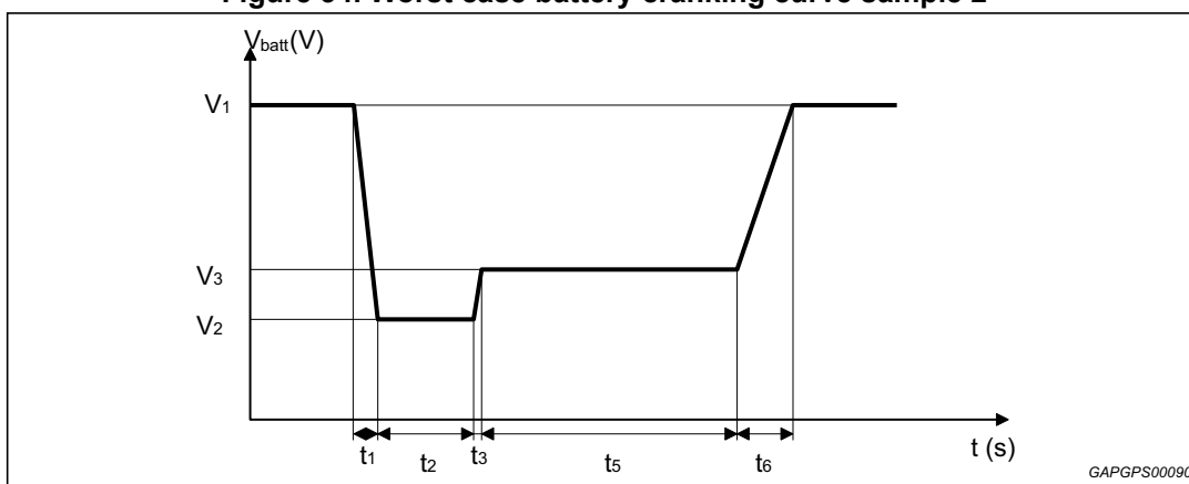
Figure 34. Worst case battery cranking curve sample 2
