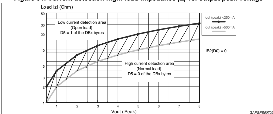
Figure 31. Current detection high: load impedance |Z| vs. output peak voltage
