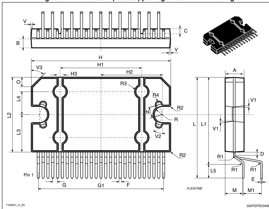
Figure 41. Flexiwatt 27 (vertical) package mechanical drawing
