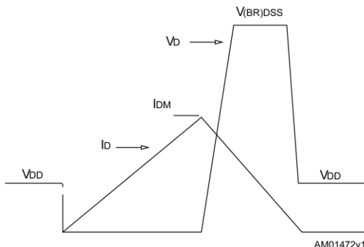
Figure 17: Unclamped inductive waveform
