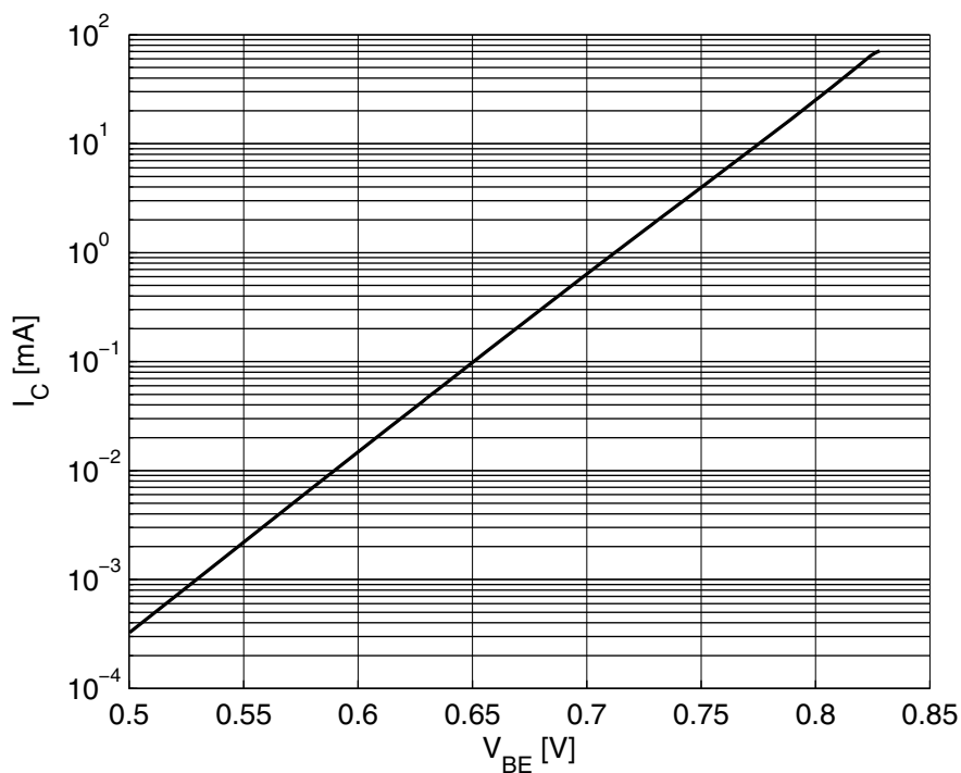
Figure 5-4 Collector Current vs. Base Emitter Voltage I_C = f(V_{BE}) , V_{CE} = 2 V
