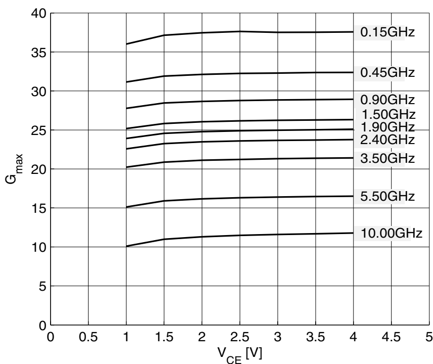
Figure 5-14 Maximum Power Gain G_{\max} = f(V_{CE}) , I_C = 30\text{ mA} , f = \text{Parameter in GHz}
