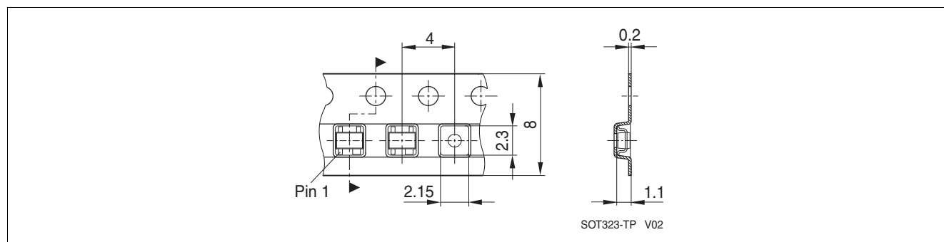
Figure 7-4 Tape Dimensions
