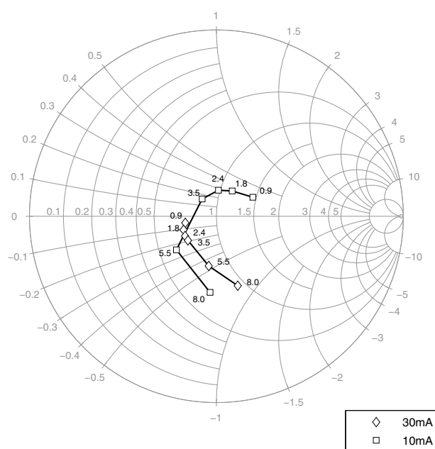
Figure 5-16 Source Impedance for Minimum Noise Figure Z_{opt} = f(f) , V_{CE} = 3\text{ V} , I_C = 10 / 30\text{ mA}
