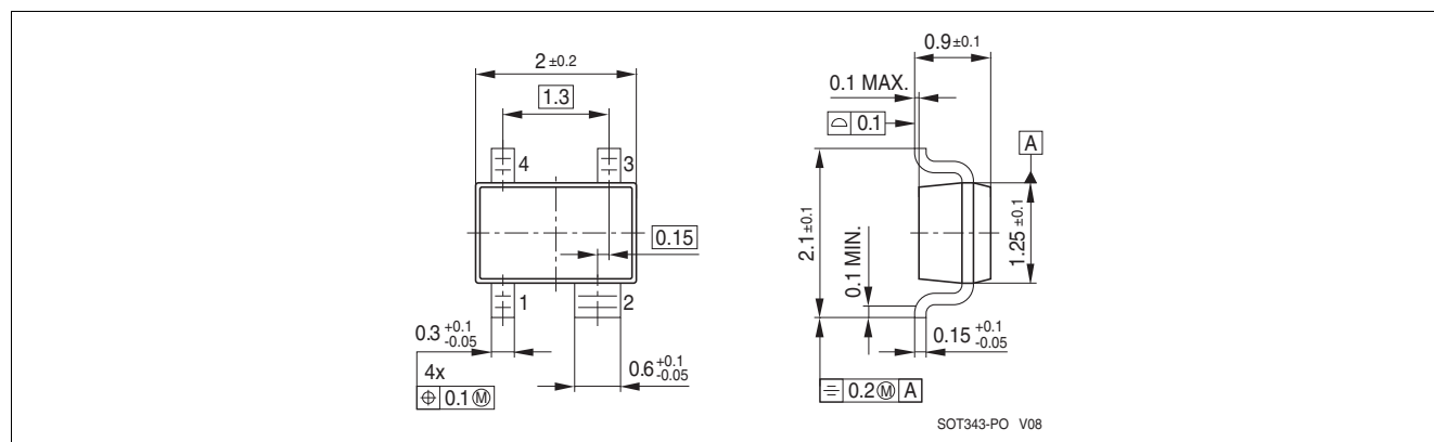
Figure 7-1 Package Outline
