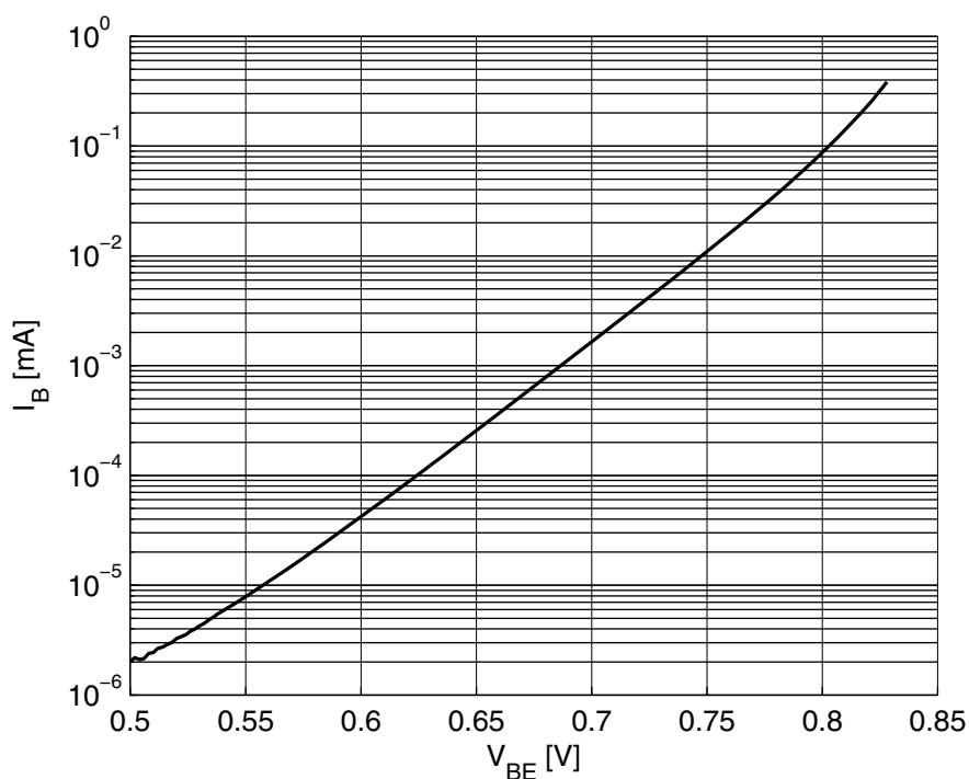
Figure 5-5 Base Current vs. Base Emitter Forward Voltage I_B = f(V_{BE}) , V_{CE} = 2 V
