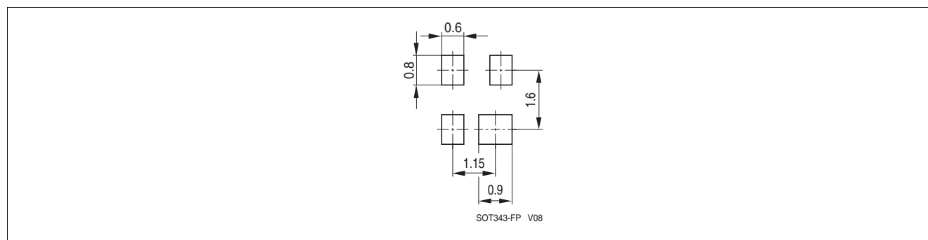
Figure 7-2 Package Footprint
