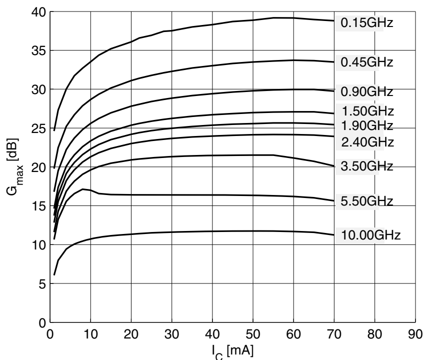
Figure 5-13 Maximum Power Gain G_{\max} = f(I_C) , V_{CE} = 3\text{ V} , f = \text{Parameter in GHz}
