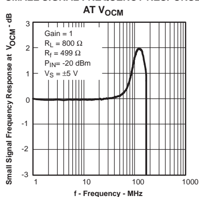
SMALL SIGNAL FREQUENCY RESPONSE
