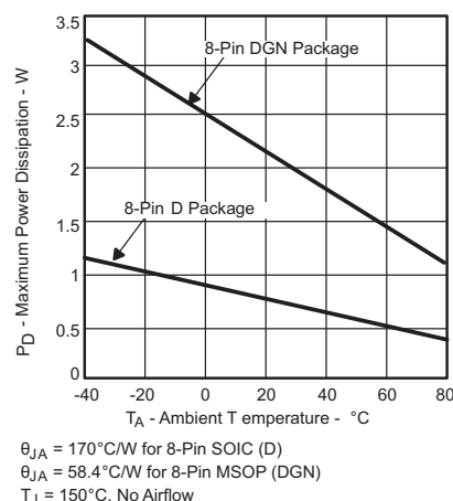
Figure 114. Maximum Power Dissipation vs Ambient Temperature
