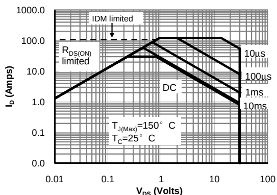
V_GS > or equal to 4.5V Figure 9: Maximum Forward Biased Safe Operating Area (Note F)
