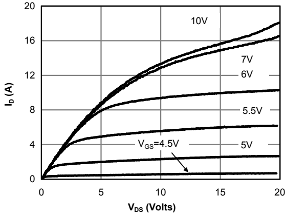
Figure 1: On-Region Characteristics@25°C
