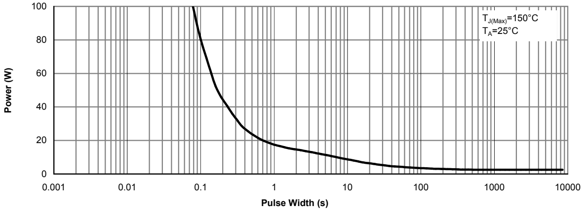
Figure 16: Single Pulse Power Rating Junction-to-Ambient (Note G)
