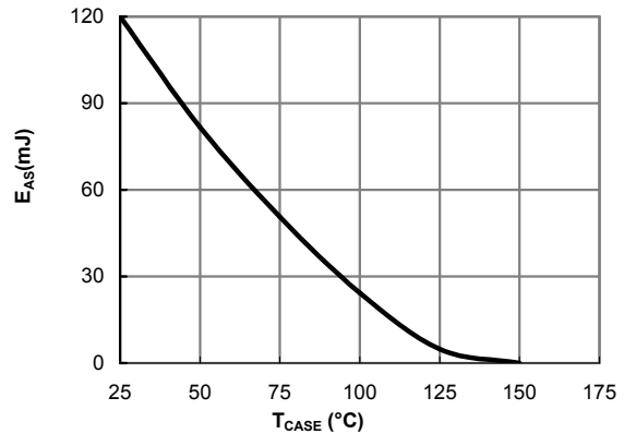
Figure 12: Avalanche energy
