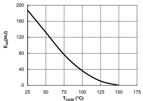
Figure 12: Avalanche energy
