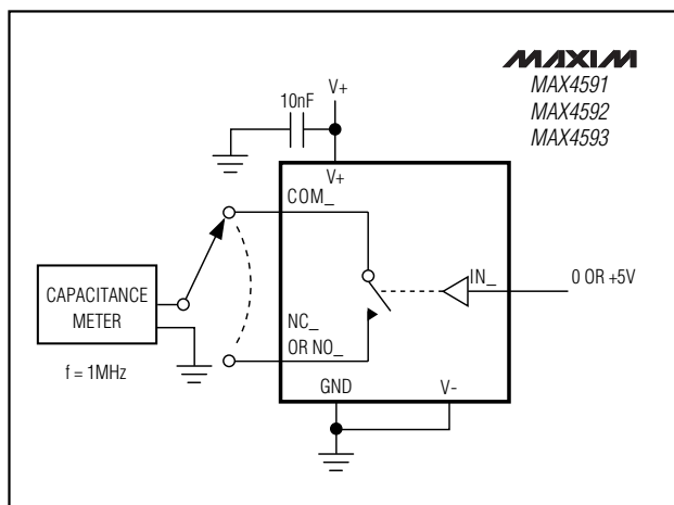
Figure 7. Channel Off-Capacitance
