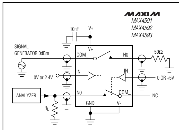
Figure 6. Crosstalk
