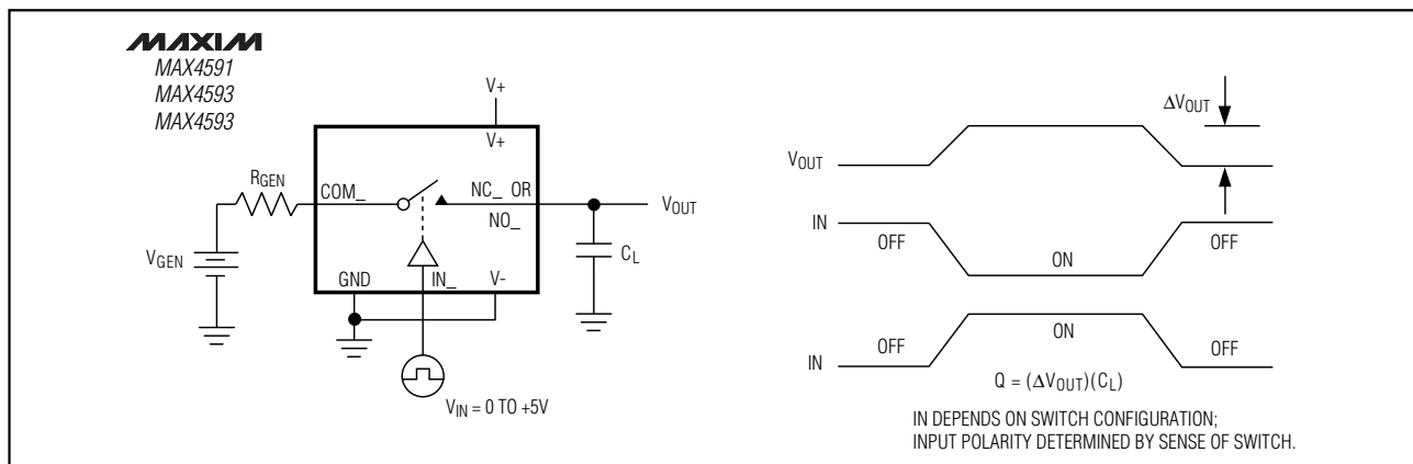
Figure 4. Charge Injection
