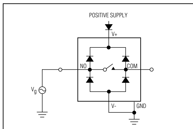
Figure 1. Overvoltage Protection Using Two External Blocking Diodes
