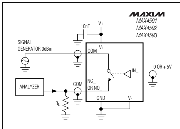
Figure 5. Off-Isolation
