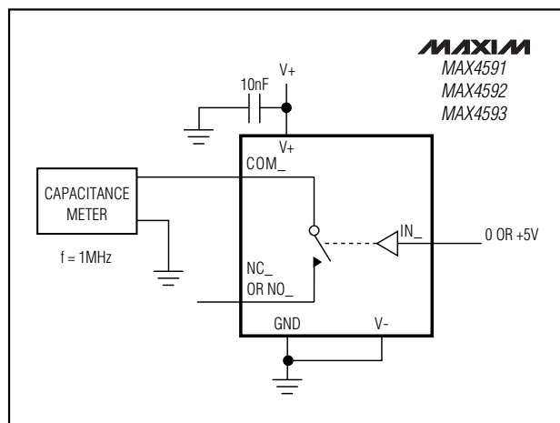
Figure 8. Channel On-Capacitance
