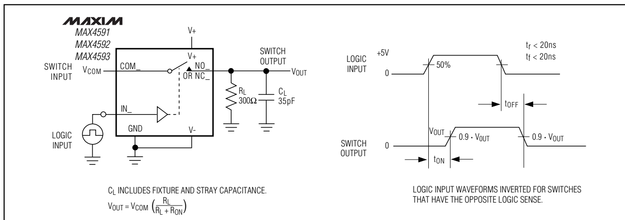
Figure 2. Switching Time
