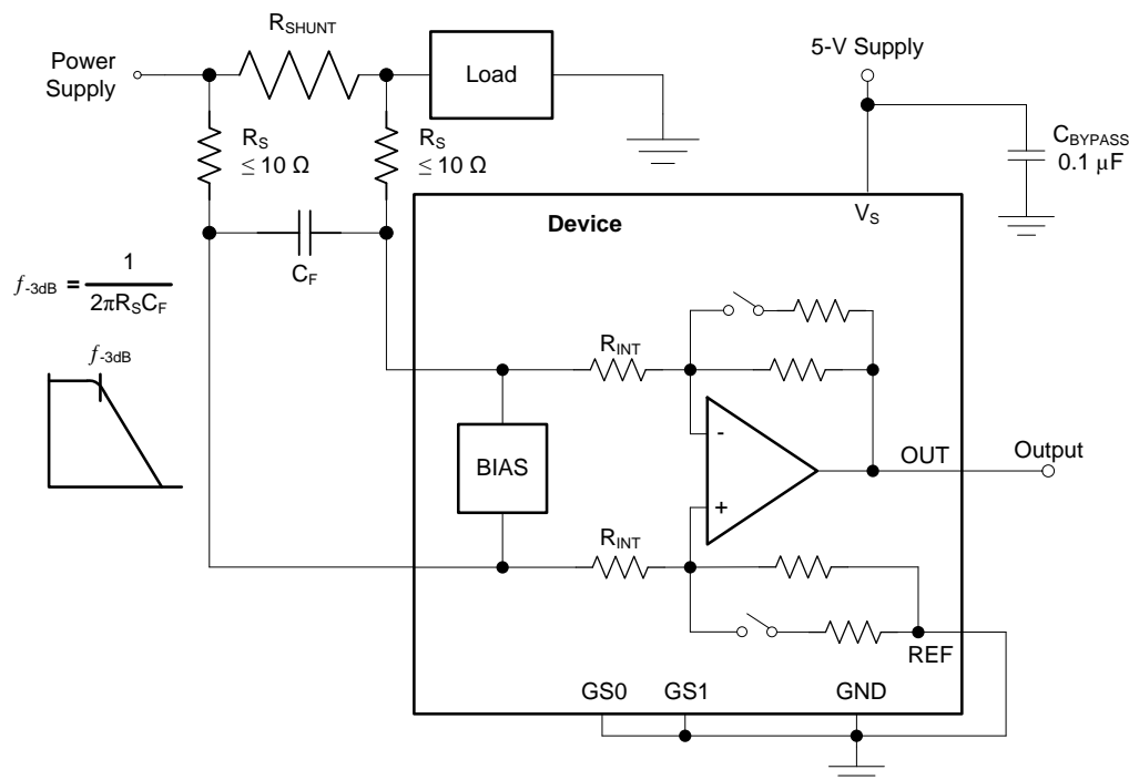
Figure 36. Input Filter
