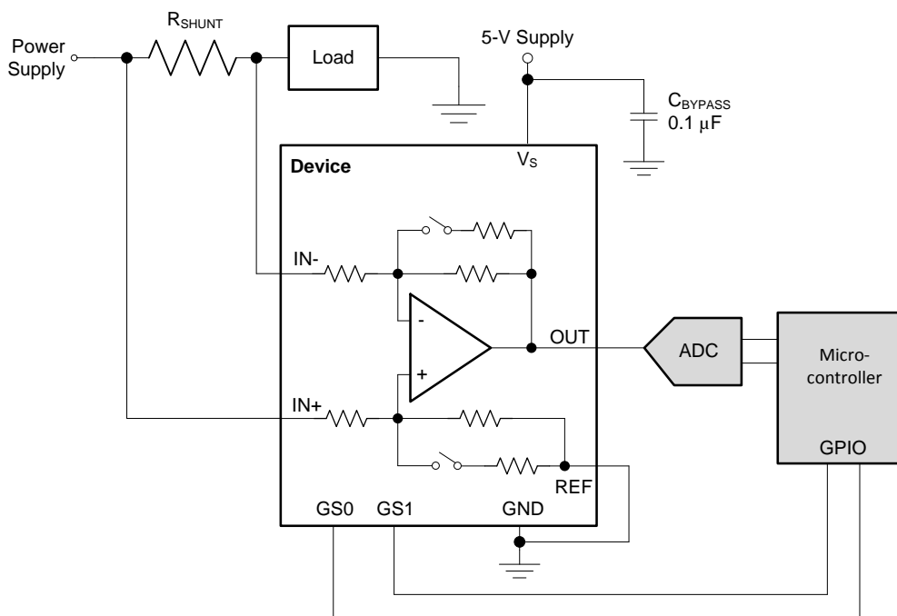
Figure 39. Microcontroller-Configured Gain Selection Schematic
