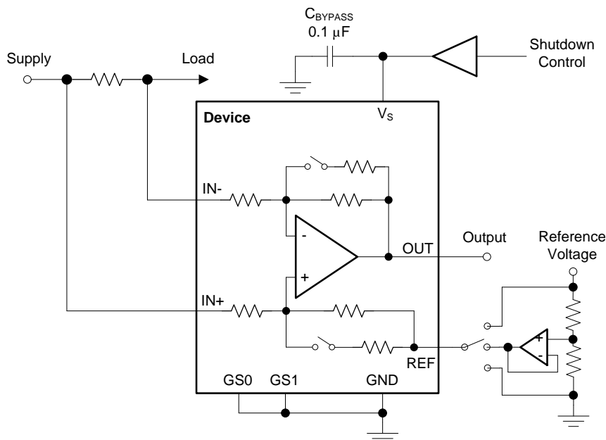
Figure 37. Shutting Down the Device
