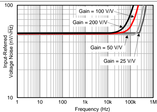
Figure 20. Input-Referred Voltage Noise vs Frequency
