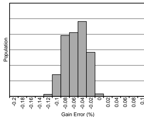
Figure 8. Gain Error Production Distribution (Gain = 200 V/V)
