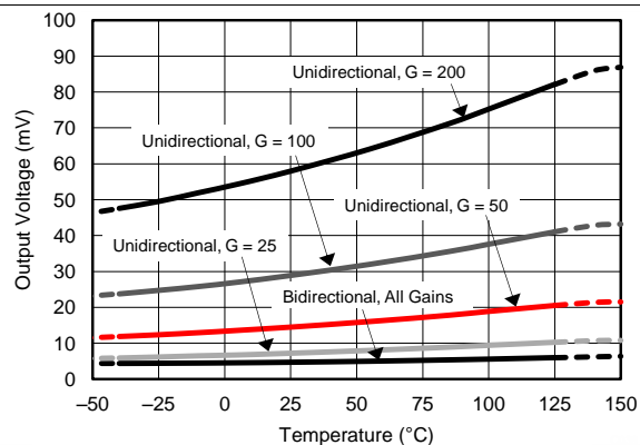
Figure 14. Unidirectional Output Voltage Swing vs. Temperature
