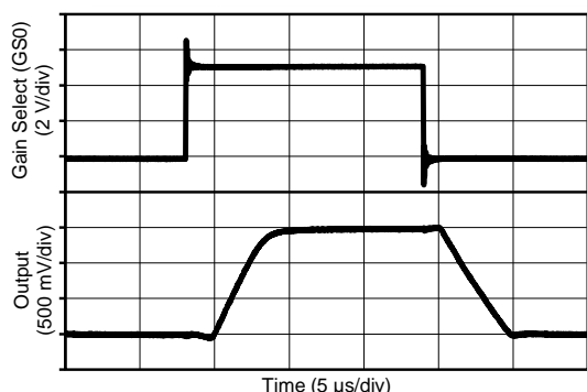
Figure 25. Step Response (Gain = 200 V/V, 2- V_{PP} Output Step)
