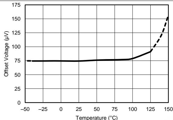
Figure 2. Input Offset Voltage vs Temperature
