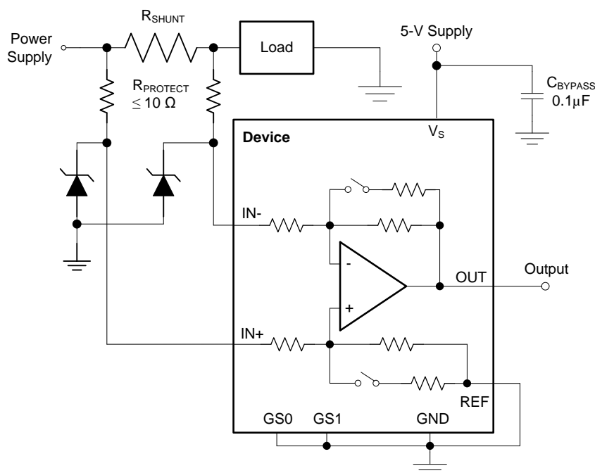
Figure 38. Device Transient Protection
