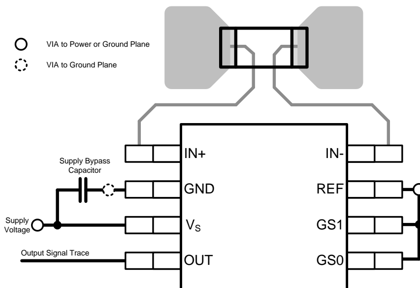
Figure 45. Recommended Layout
