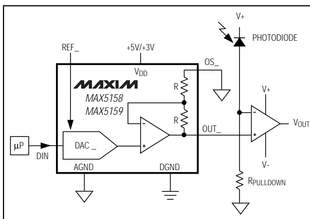
Figure 13. Digital Calibration
