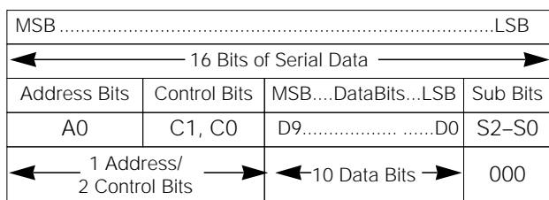
Figure 4. Serial-Data Format
