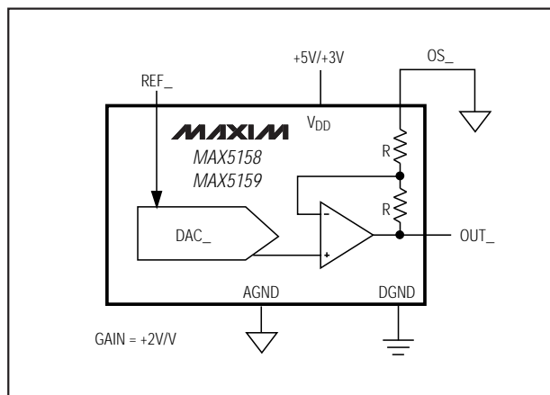
Figure 9. Unipolar Output Circuit (Rail-to-Rail)
