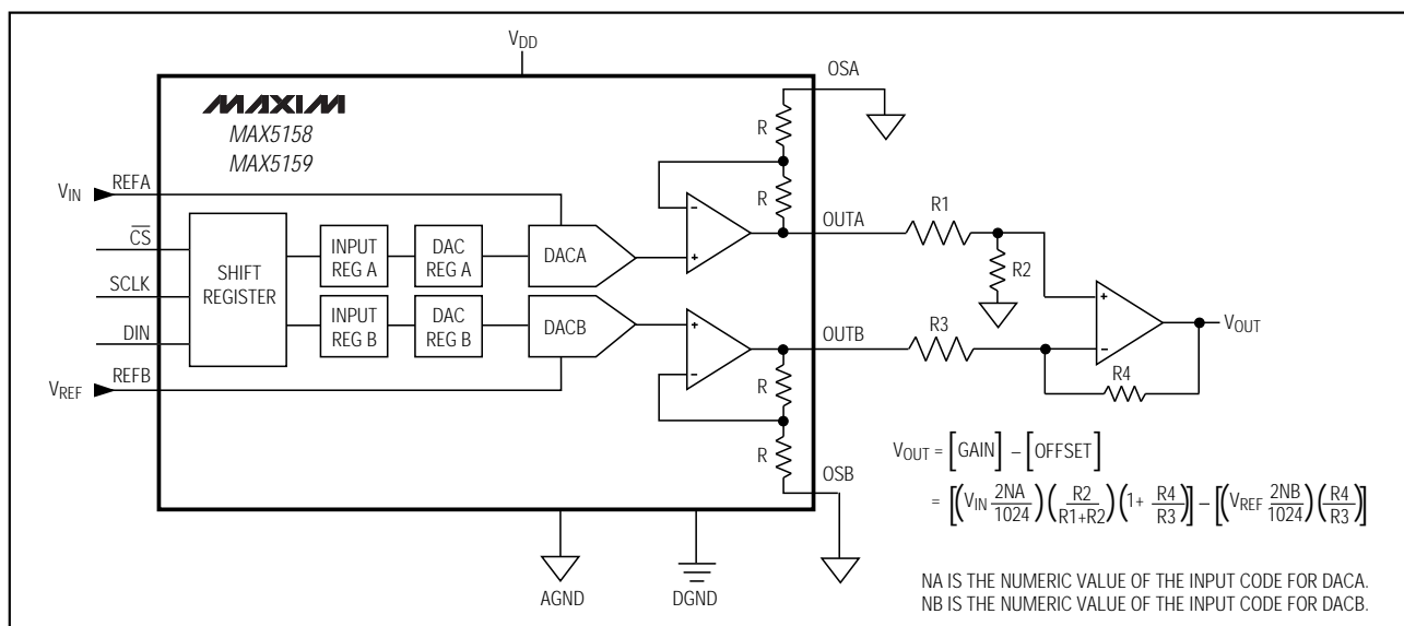
Figure 14. Digital Control of Gain and Offset
