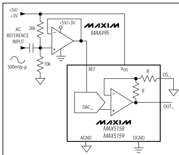
Figure 12. AC Reference Input Circuit
