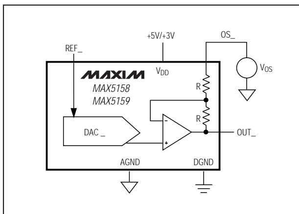
Figure 10. Setting OS_ for Output Offset
