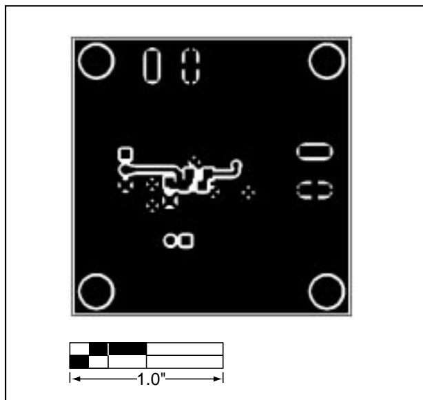
Figure 5. MAX606 EV Kit PC Board Layout—Solder Side
