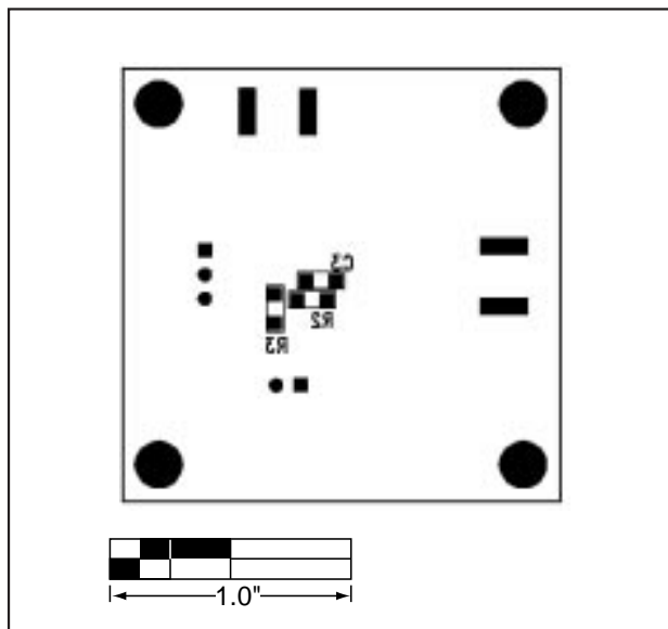
Figure 3. MAX606 EV Kit Component Placement Guide—Solder Side
