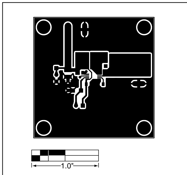
Figure 4. MAX606 EV Kit PC Board Layout—Component Side
