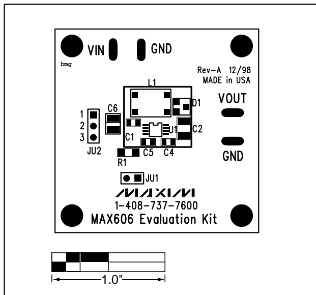
Figure 2. MAX606 EV Kit Component Placement Guide—Component Side
