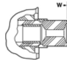
VIEW D ENLARGED FOR COAXIAL USE ONLY
