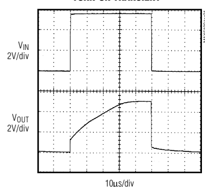
MAX6195 TURN-ON TRANSIENT
