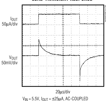
MAX6195 LOAD-TRANSIENT RESPONSE
